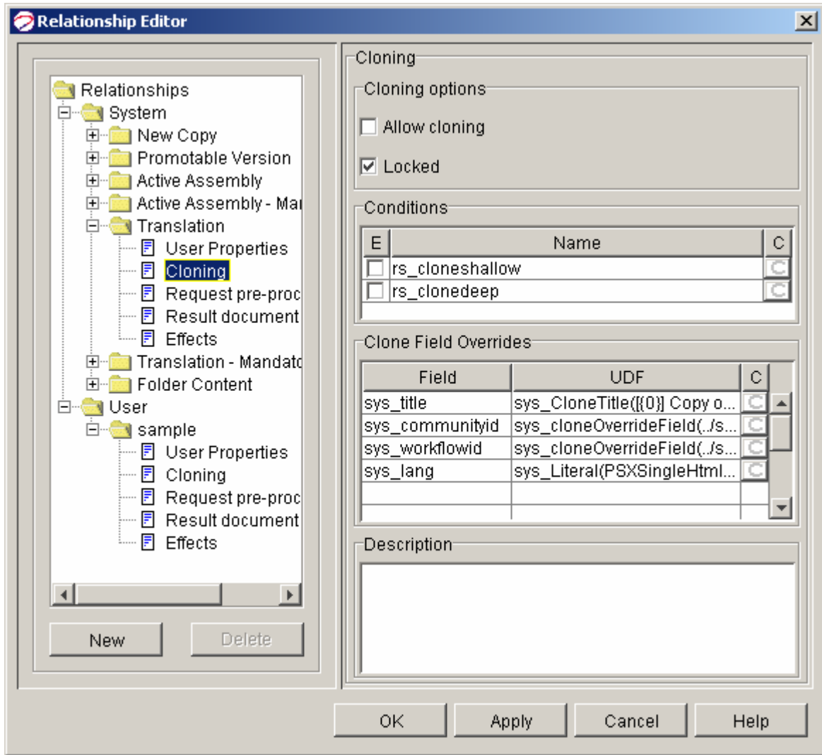
Figure 28: Default Cloning Configuration of the Translation Relationship
