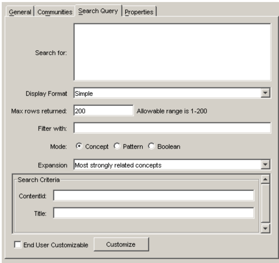
Figure 78: Search Query Tab in View and Search Editor Illustrating the Allowable Range Text
