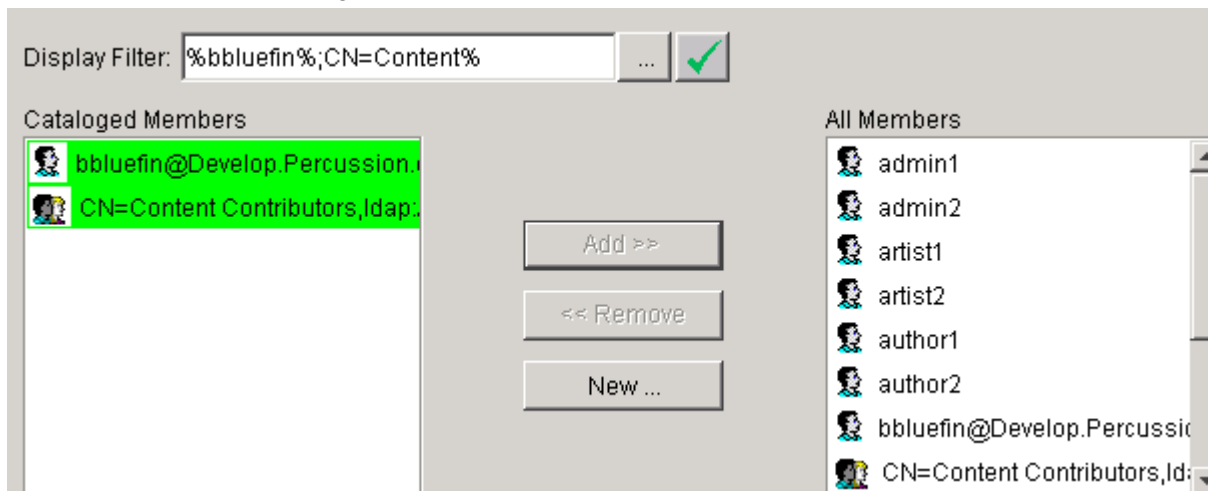
Figure 59: Cataloged Members Added to Default Role
