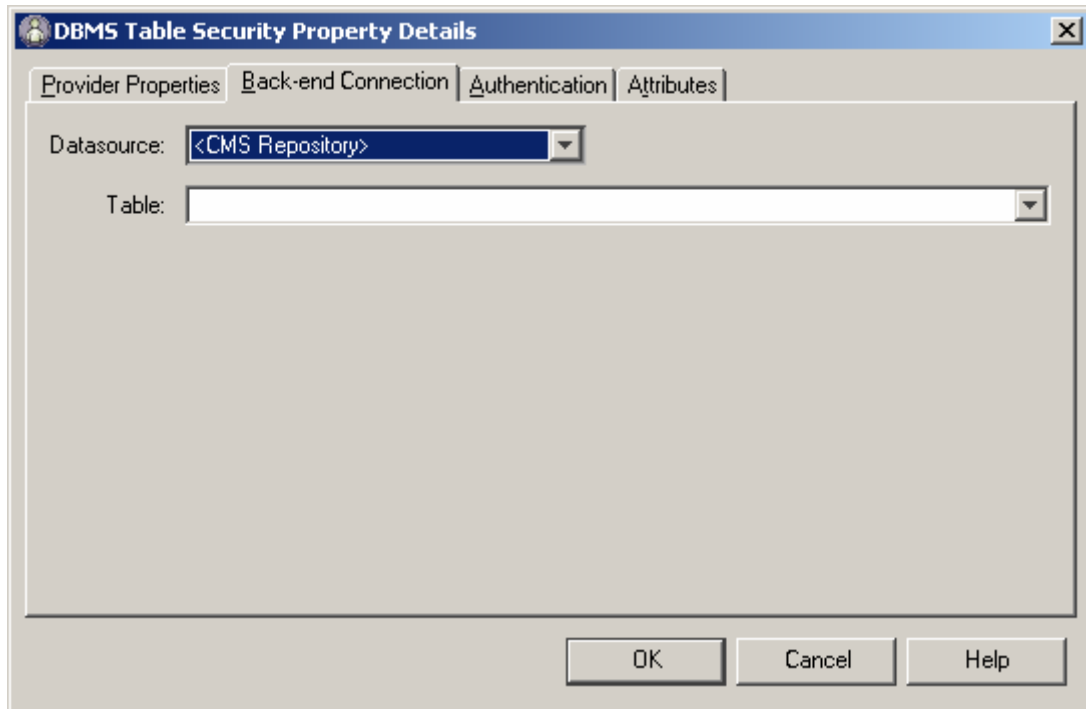
Figure 20: DBMS Table Security Property Provider Backend Connection Tab.
