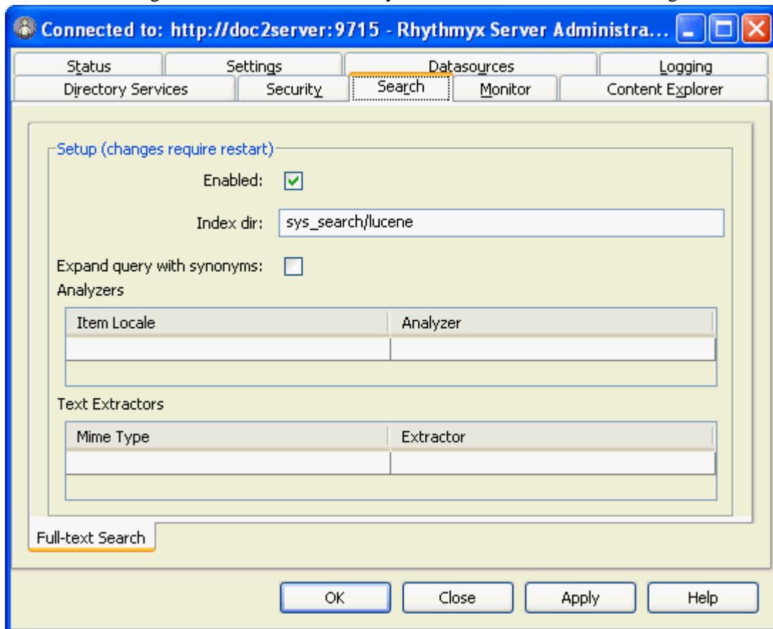
Figure 72: Search Tab
