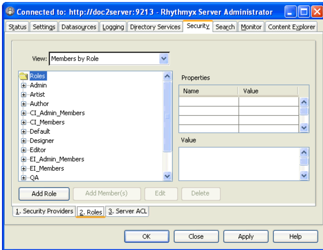
Figure 68: Roles Tab
