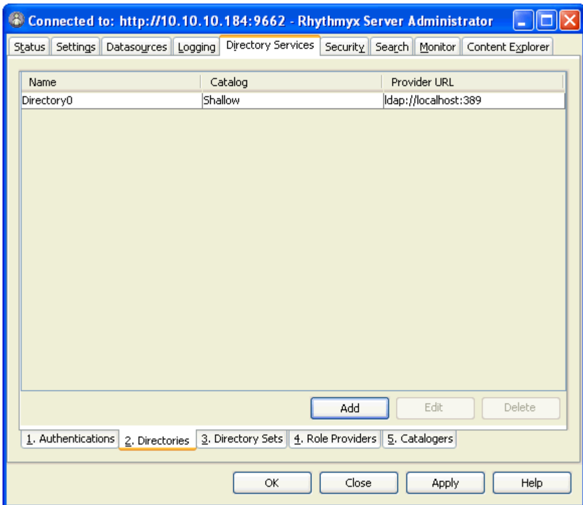
Figure 29: Directories Tab
