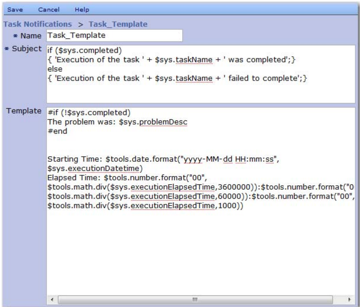
Figure 15: Task_Template
