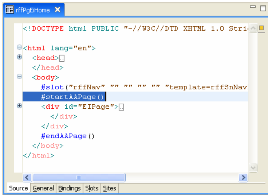
Figure 137: Page Template showing the #startAAPage and #endAAPage macros used when the Template does not have a Global Template
